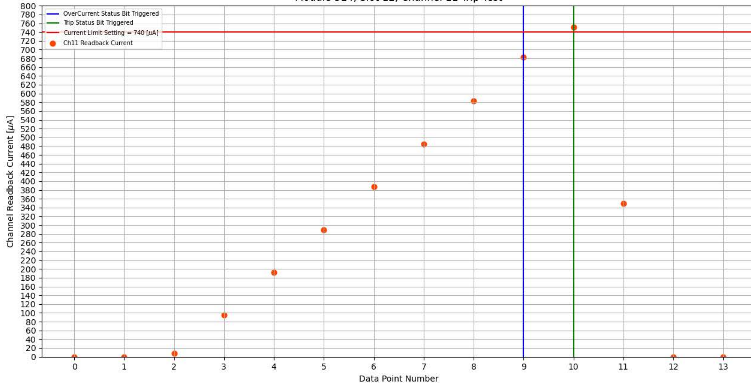
Module 314, Slot 12, Channel 11 Trip Test
