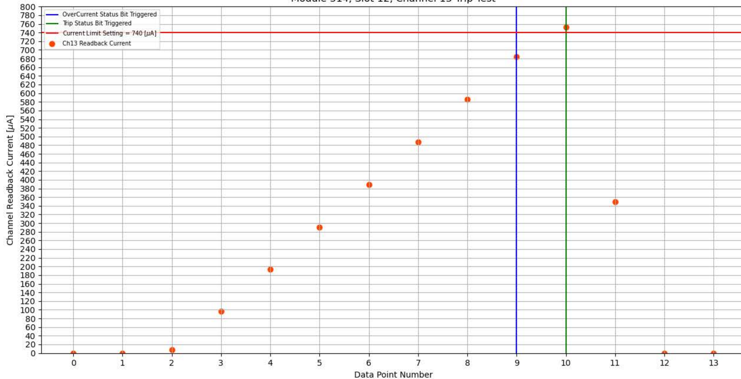
Module 314, Slot 12, Channel 13 Trip Test
