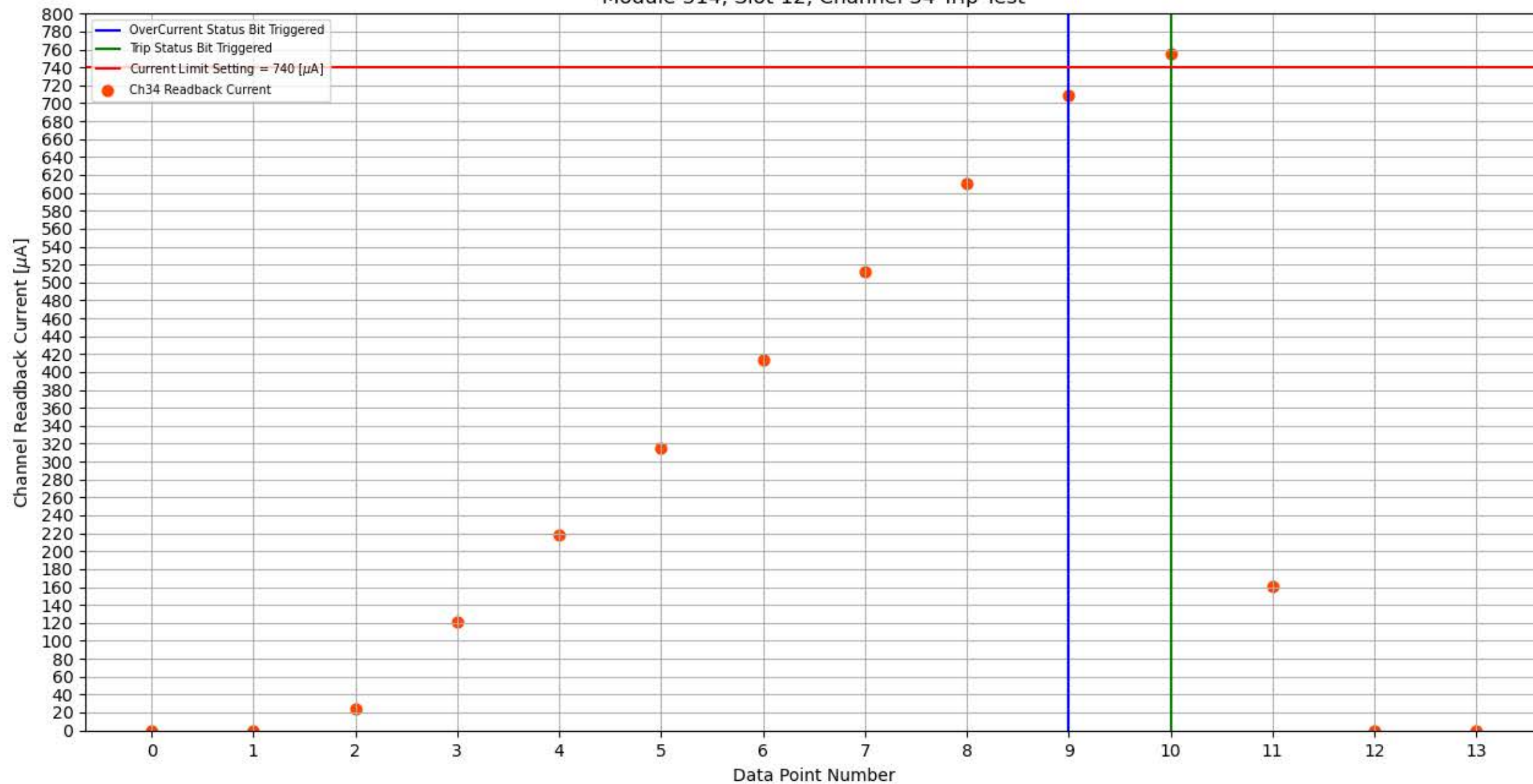
Module 314, Slot 12, Channel 34 Trip Test
