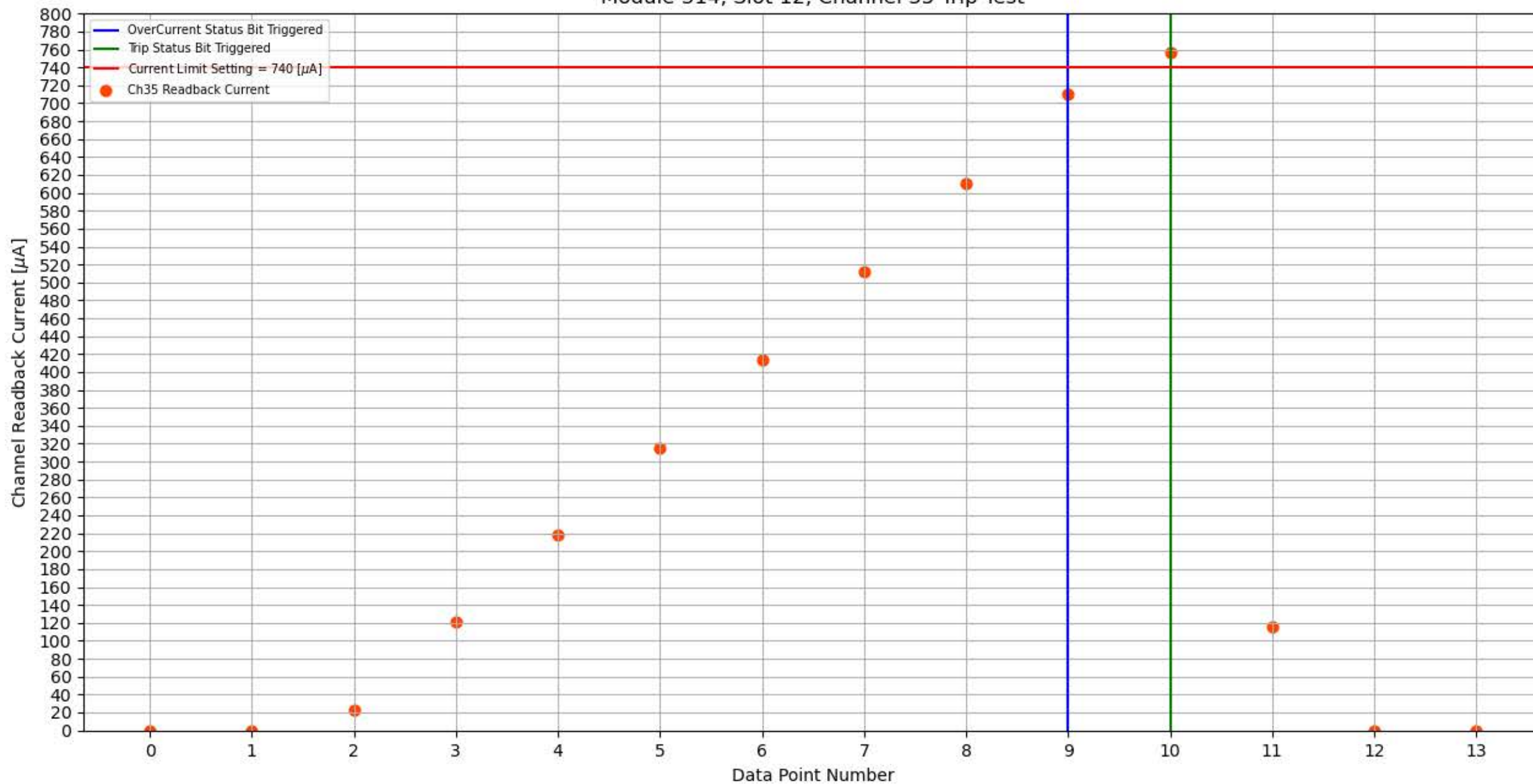
Module 314, Slot 12, Channel 35 Trip Test
