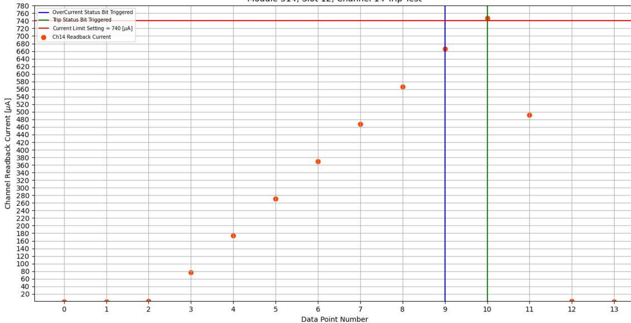
Module 314, Slot 12, Channel 14 Trip Test
