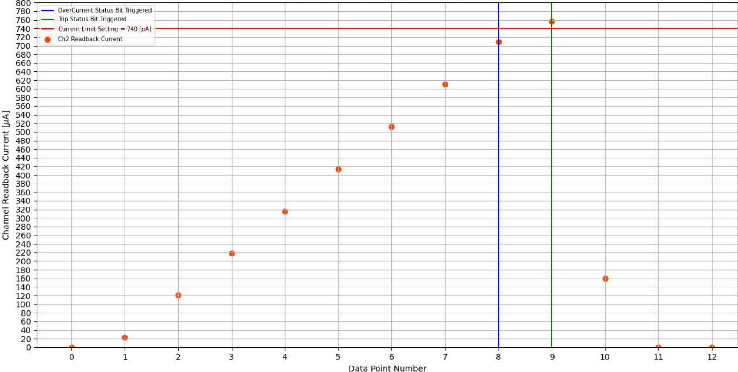
Module 314, Slot 12, Channel 2 Trip Test
