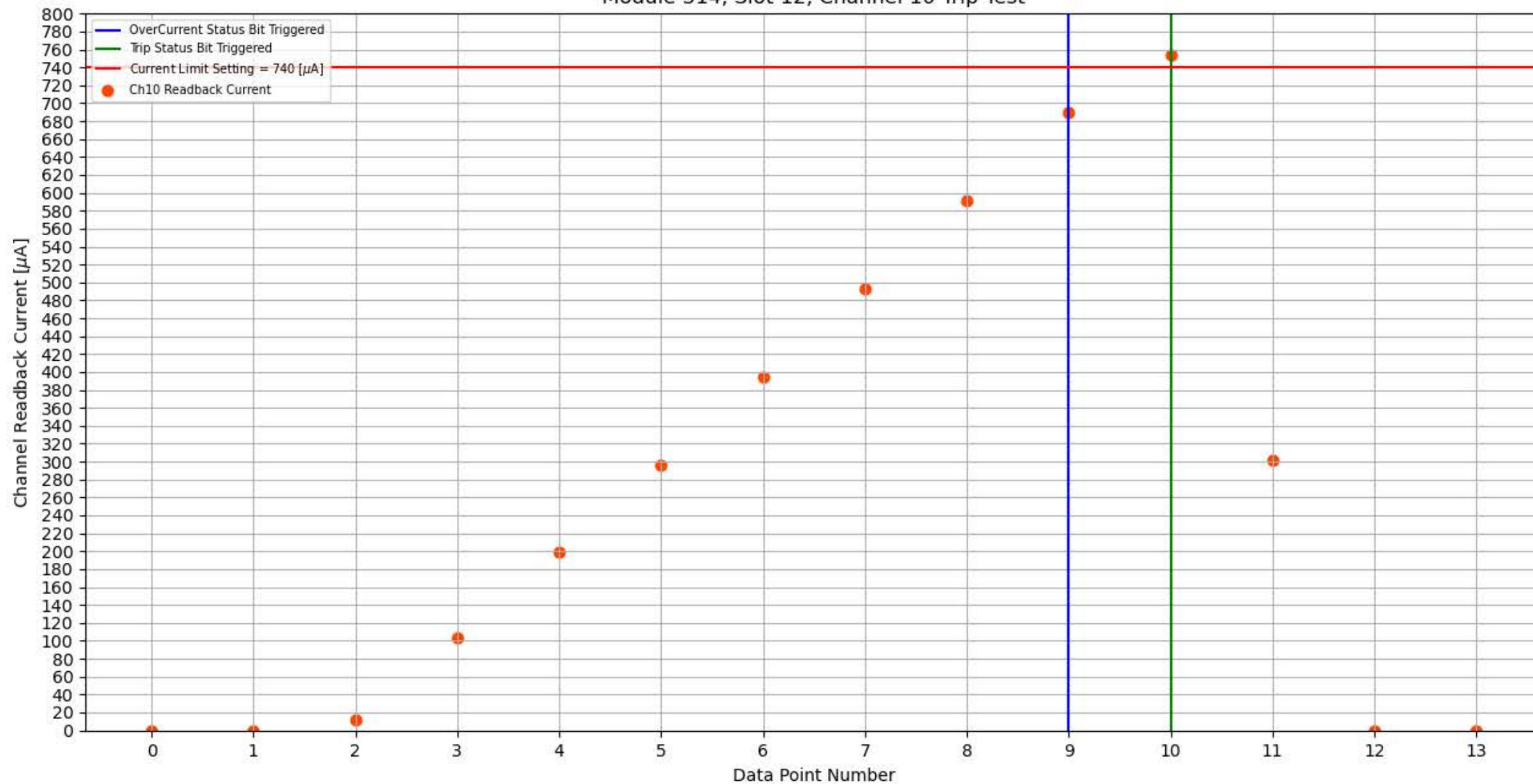
Module 314, Slot 12, Channel 10 Trip Test
