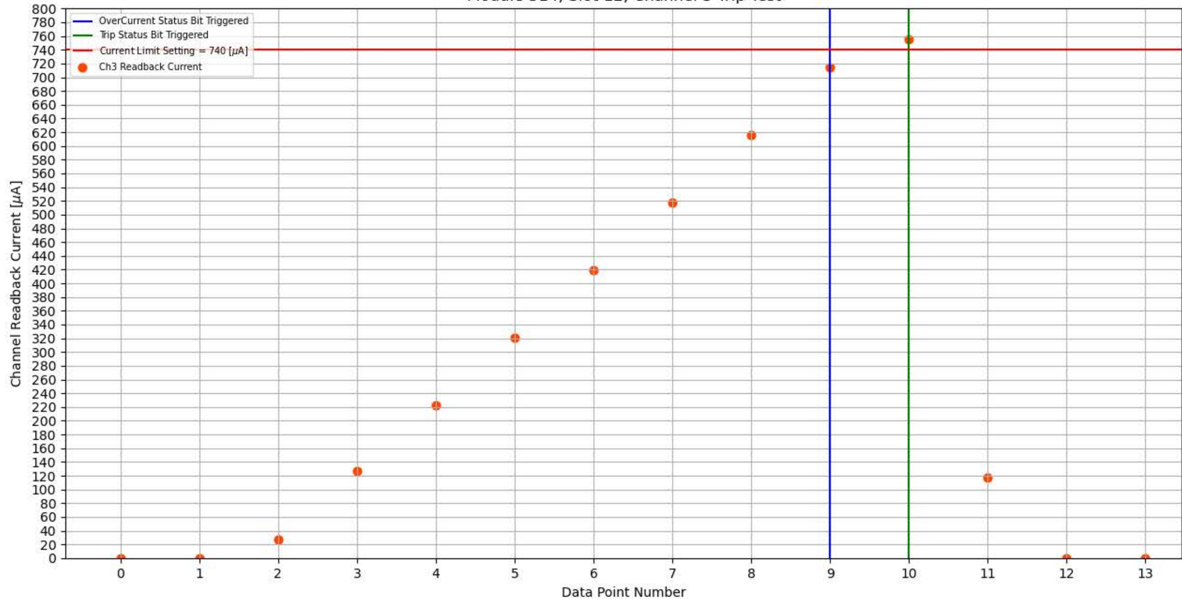
Module 314, Slot 12, Channel 3 Trip Test
