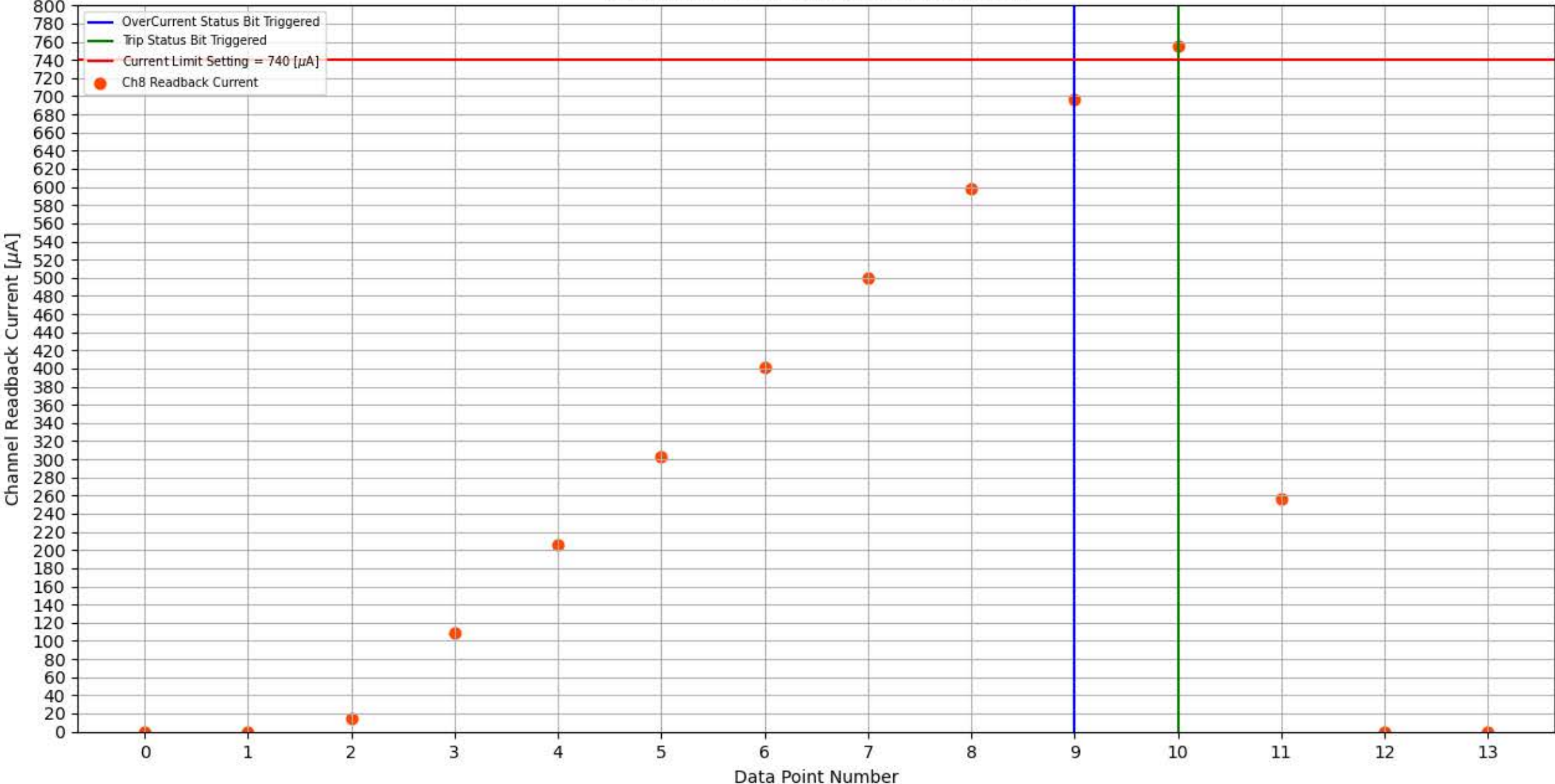
Module 314, Slot 12, Channel 8 Trip Test
