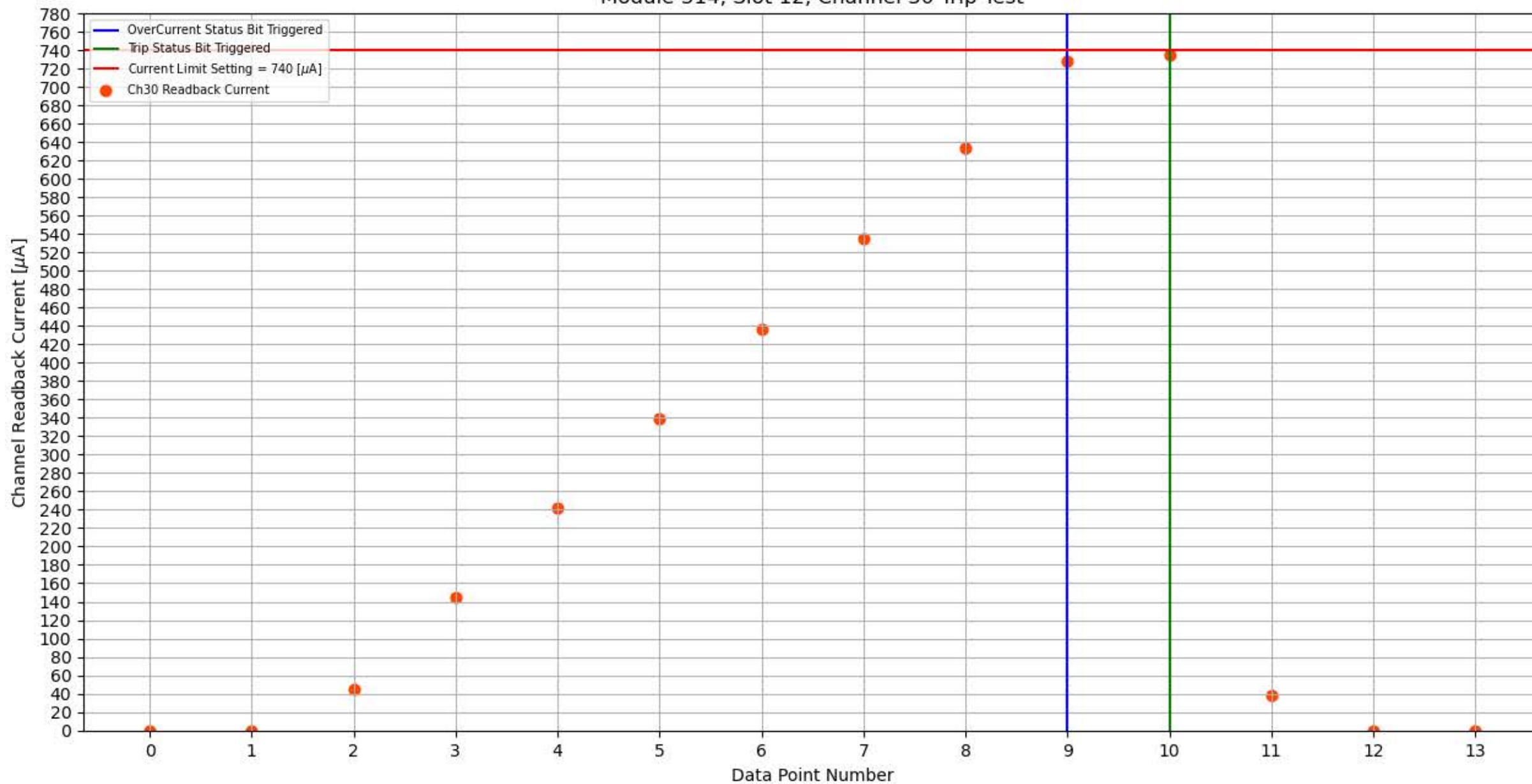
Module 314, Slot 12, Channel 30 Trip Test
