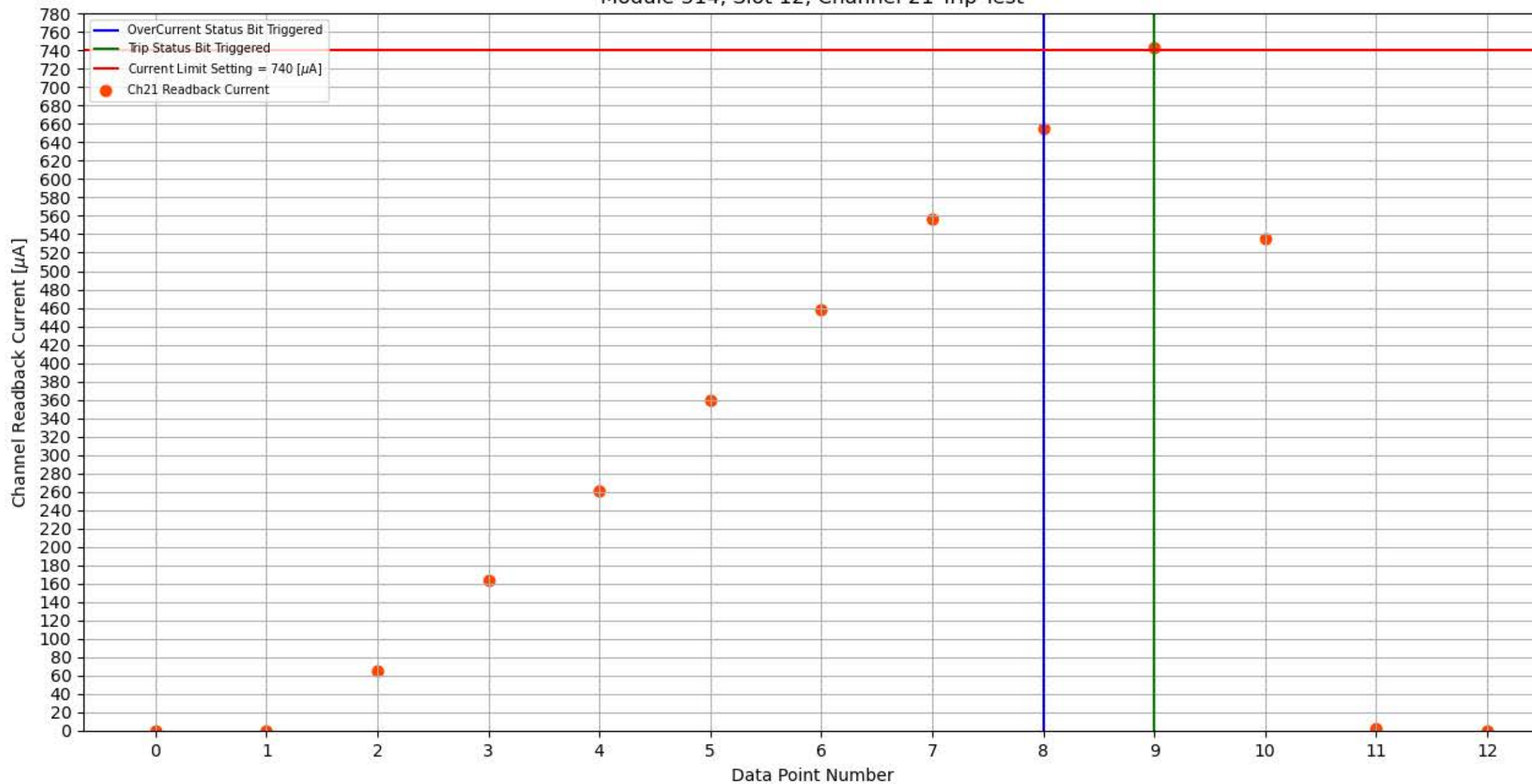
Module 314, Slot 12, Channel 21 Trip Test
