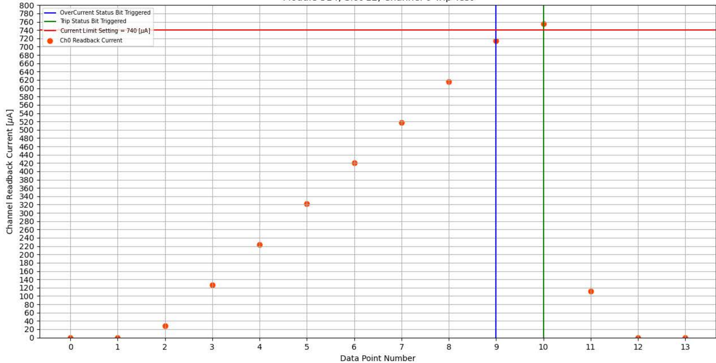
Module 314, Slot 12, Channel 0 Trip Test
