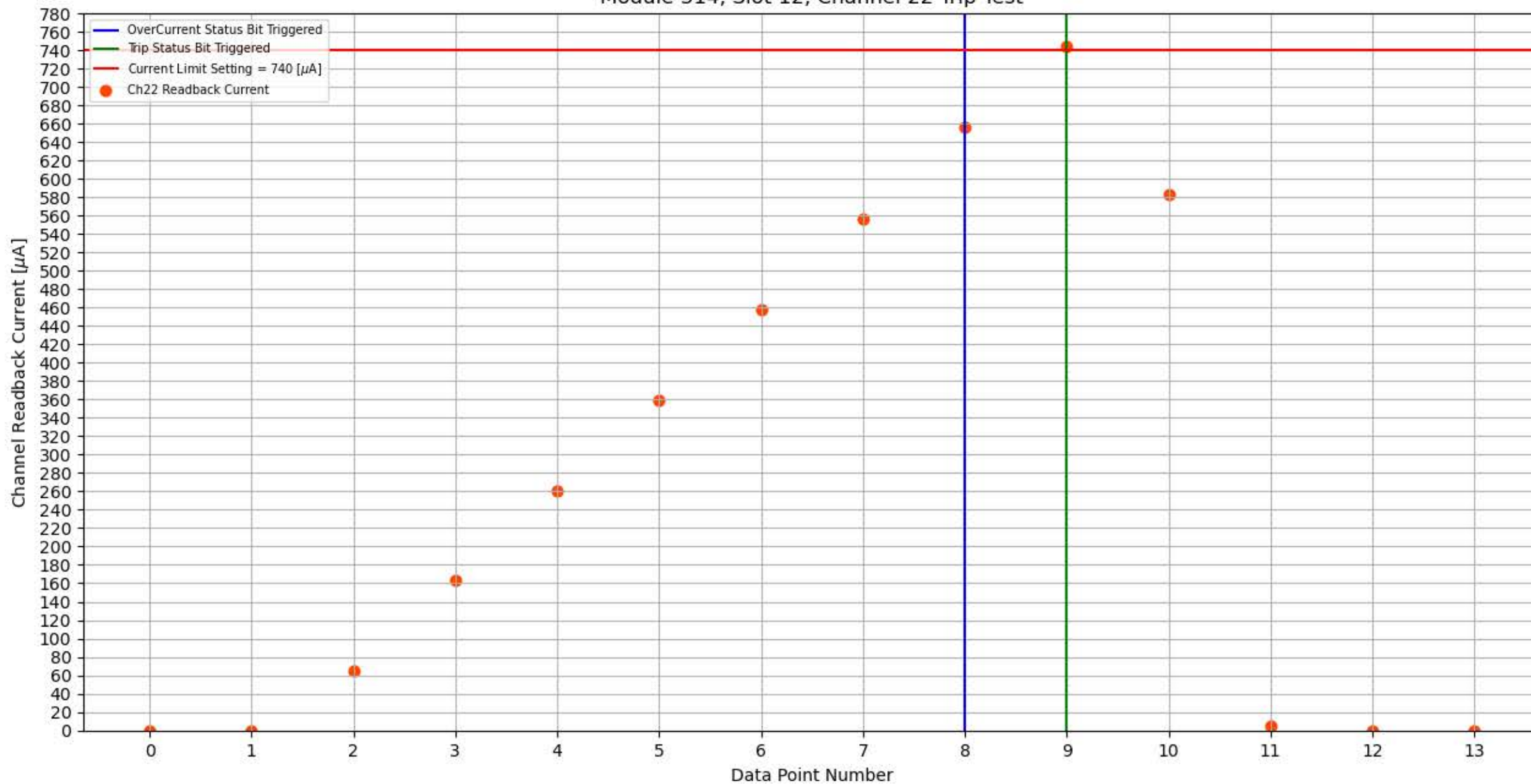
Module 314, Slot 12, Channel 22 Trip Test
