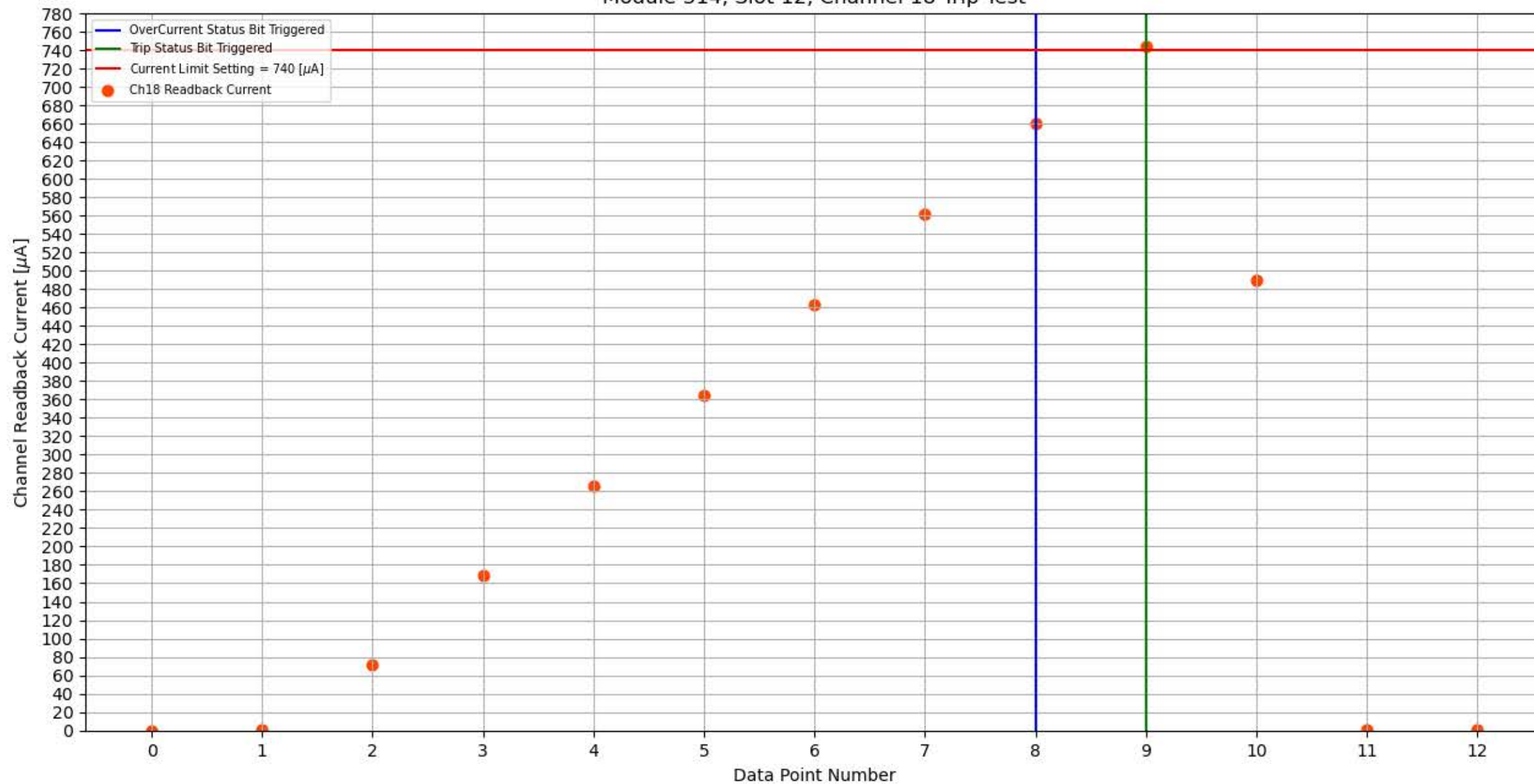
Module 314, Slot 12, Channel 18 Trip Test
