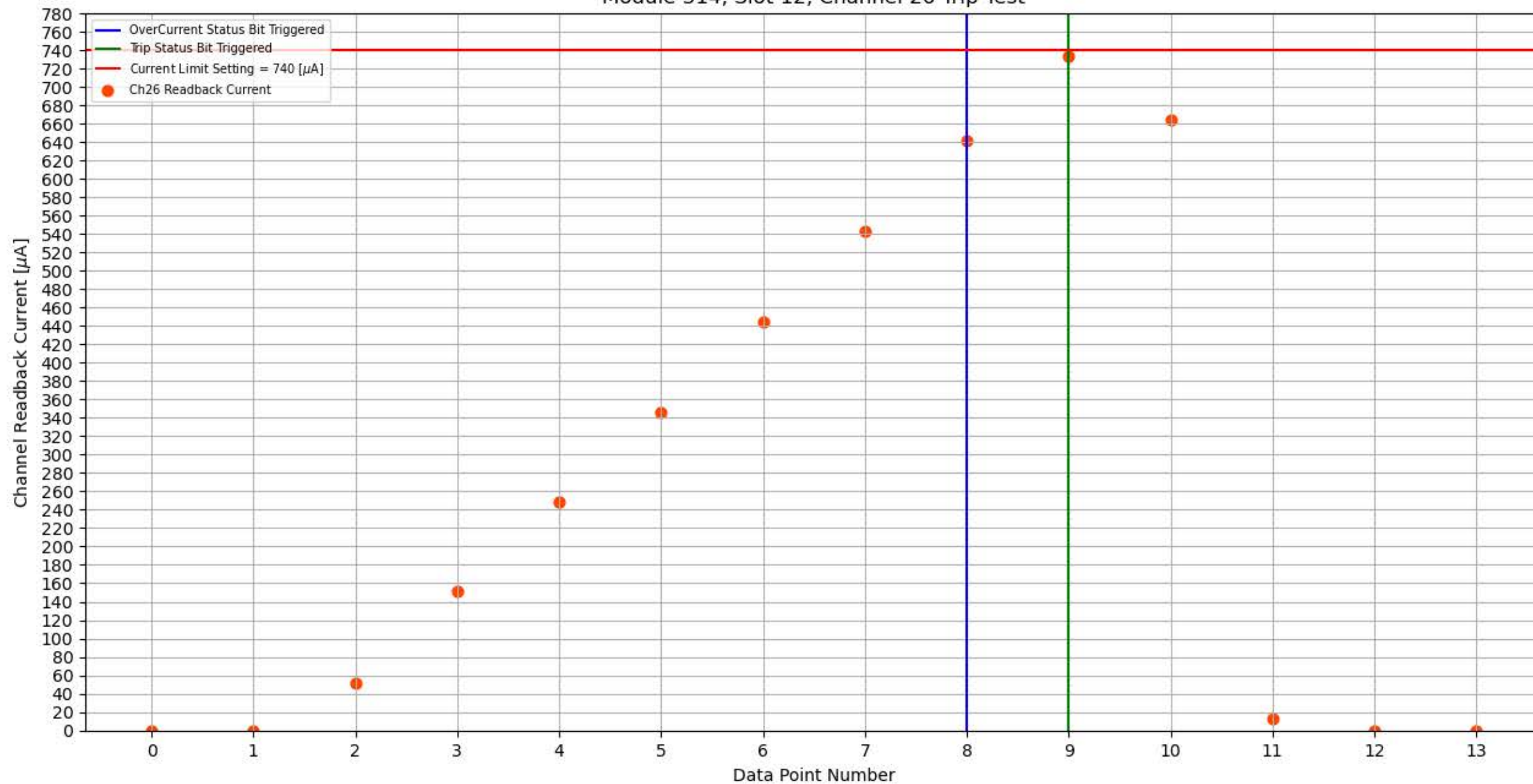
Module 314, Slot 12, Channel 26 Trip Test
