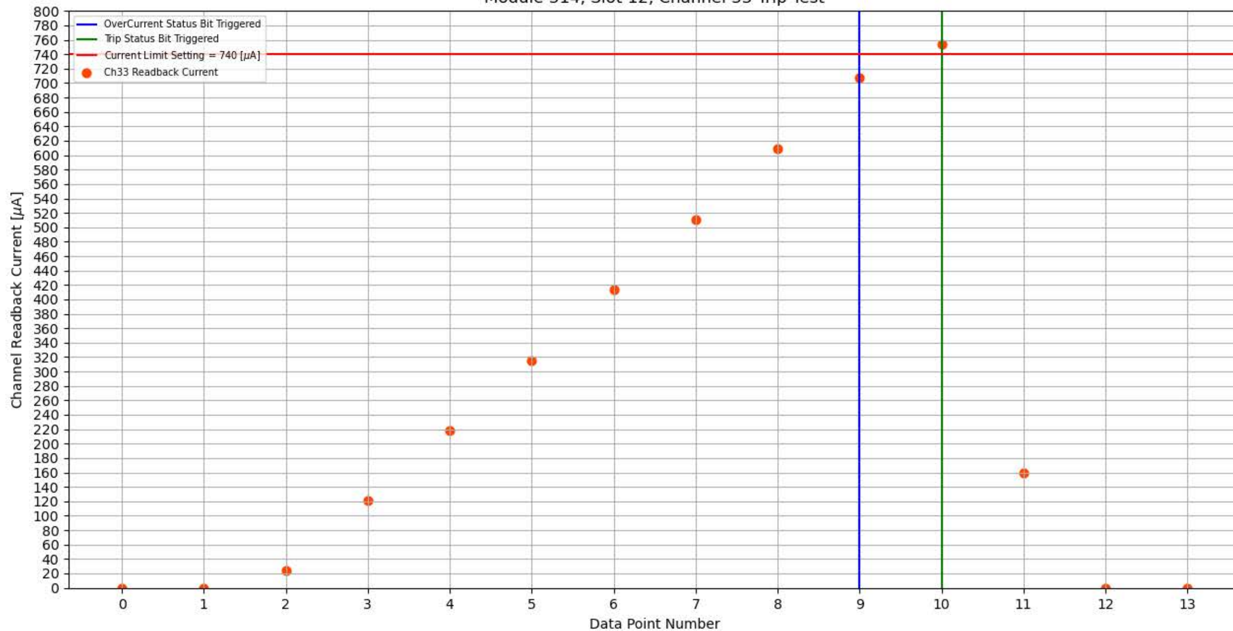
Module 314, Slot 12, Channel 33 Trip Test
