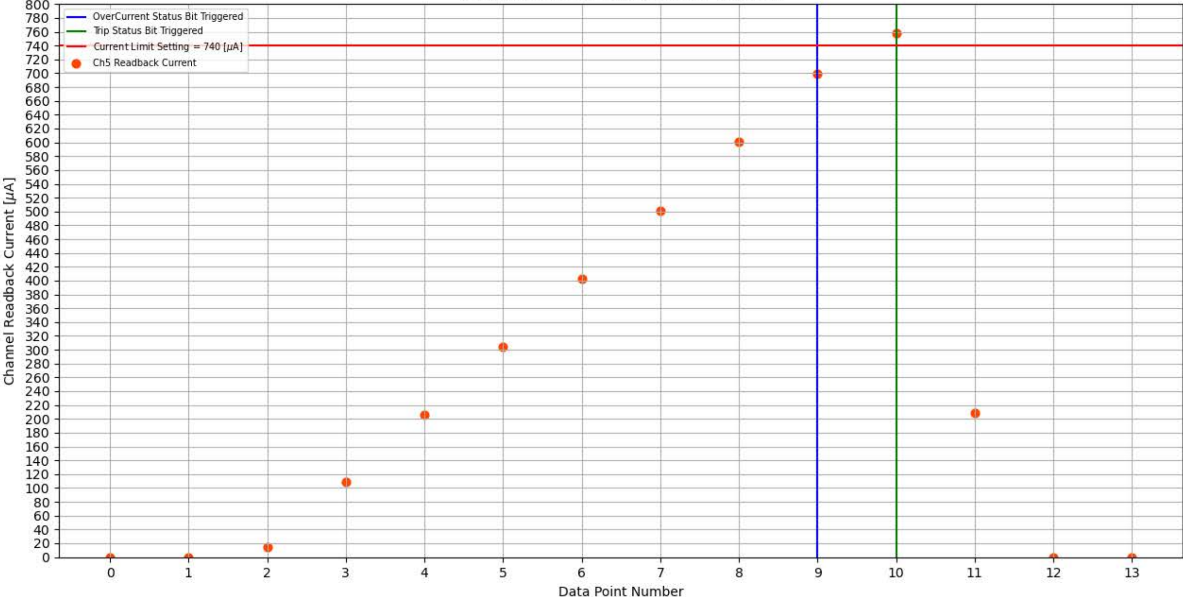
Module 314, Slot 12, Channel 5 Trip Test
