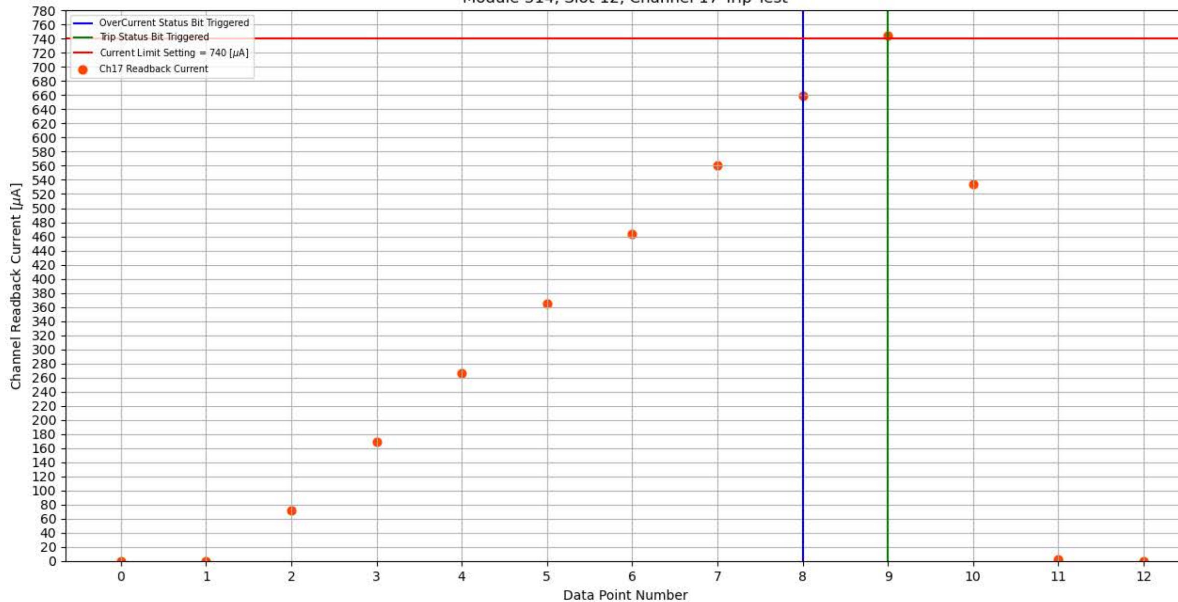
Module 314, Slot 12, Channel 17 Trip Test
