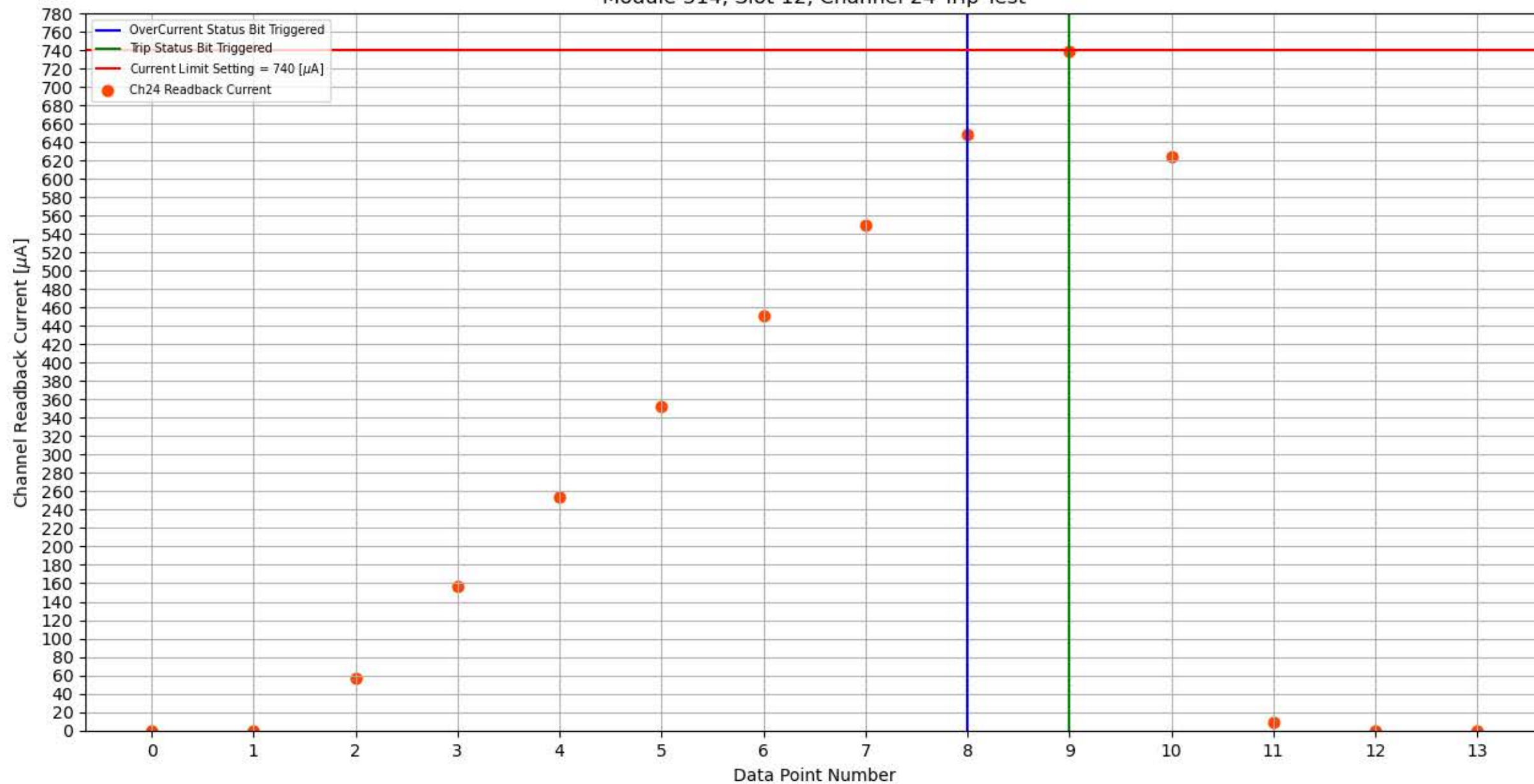
Module 314, Slot 12, Channel 24 Trip Test
