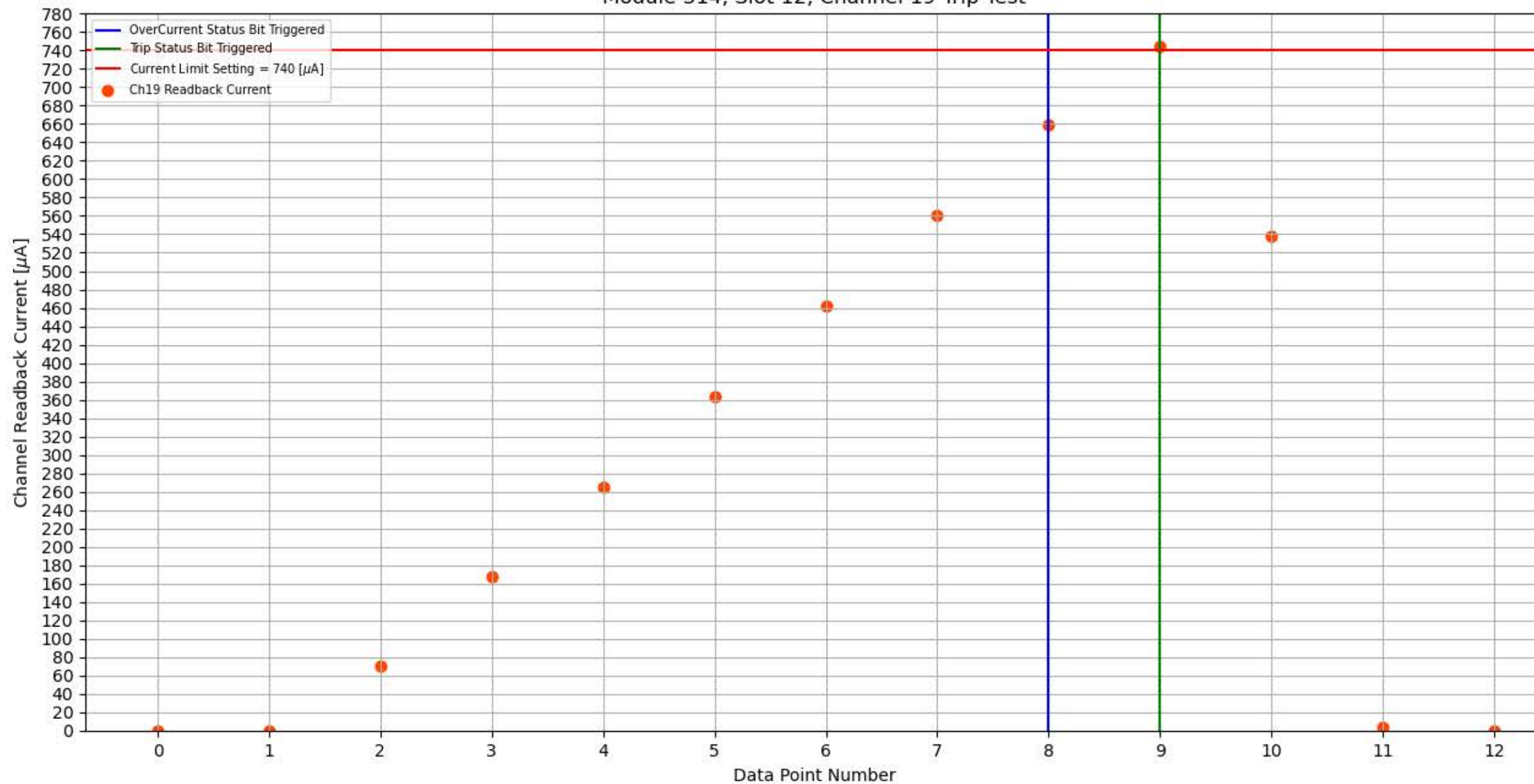
Module 314, Slot 12, Channel 19 Trip Test
