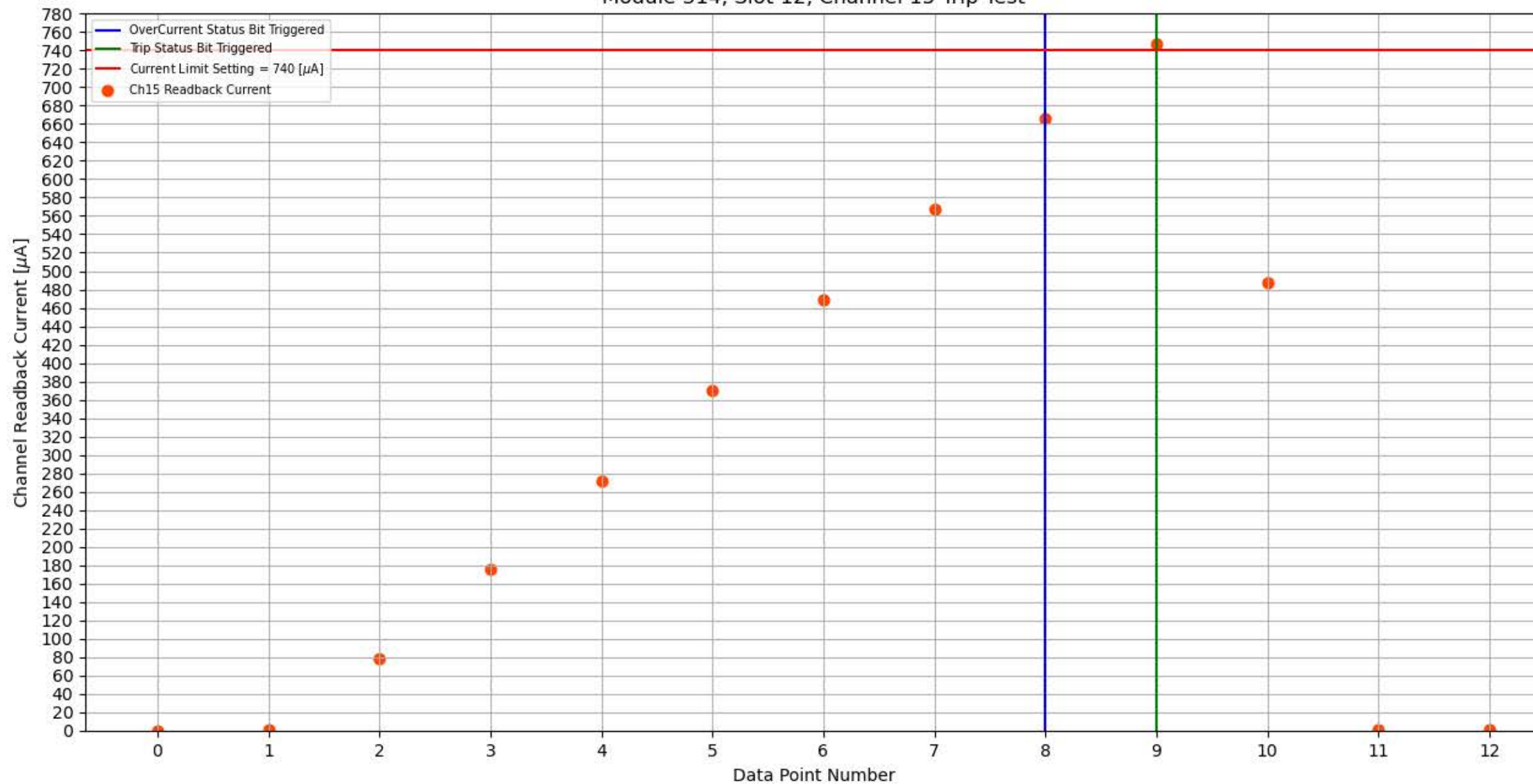
Module 314, Slot 12, Channel 15 Trip Test
