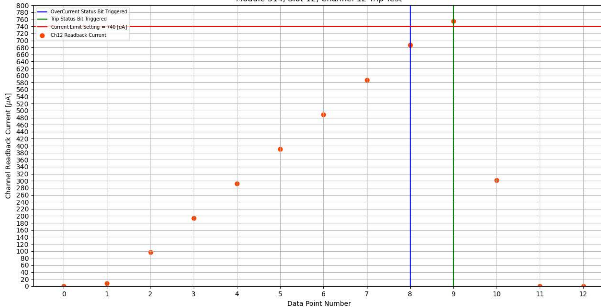
Module 314, Slot 12, Channel 12 Trip Test
