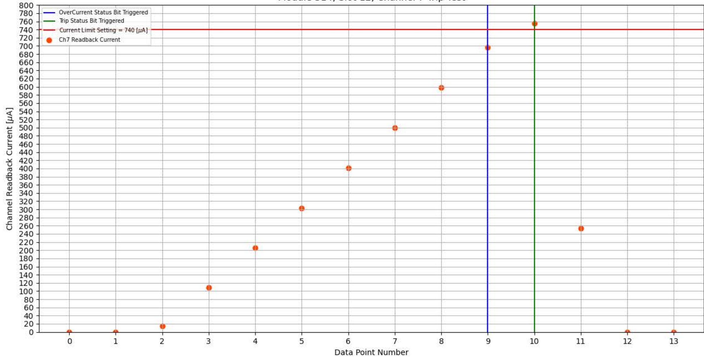
Module 314, Slot 12, Channel 7 Trip Test
