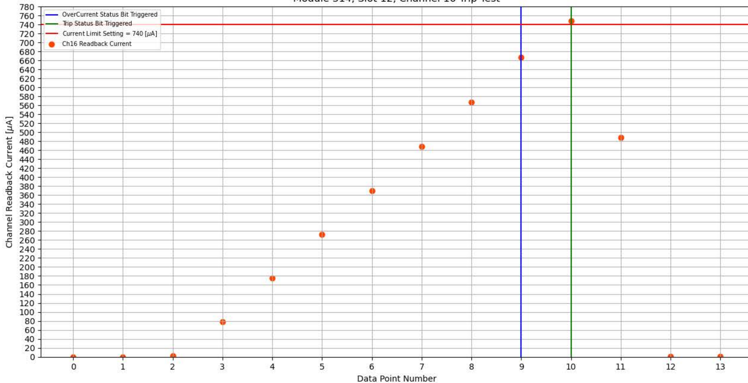
Module 314, Slot 12, Channel 16 Trip Test
