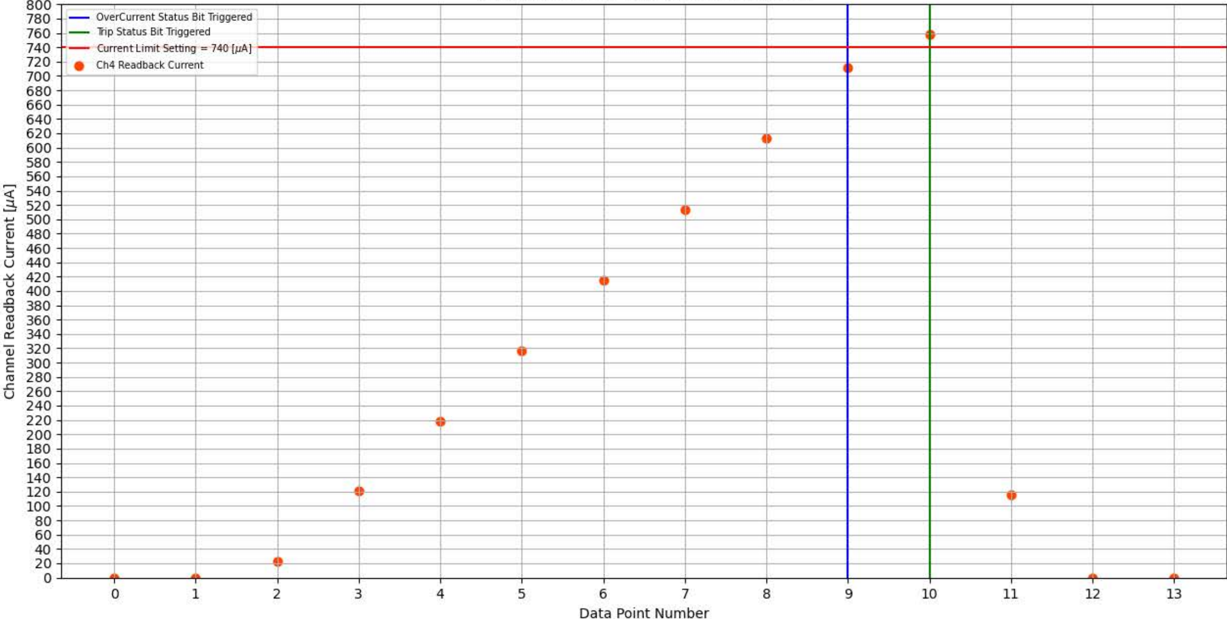
Module 314, Slot 12, Channel 4 Trip Test
