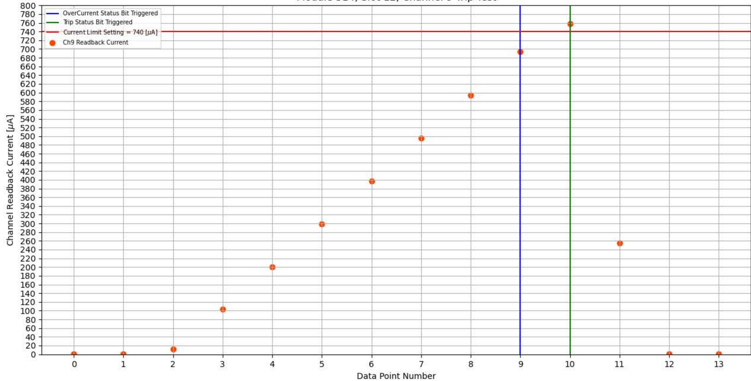
Module 314, Slot 12, Channel 9 Trip Test
