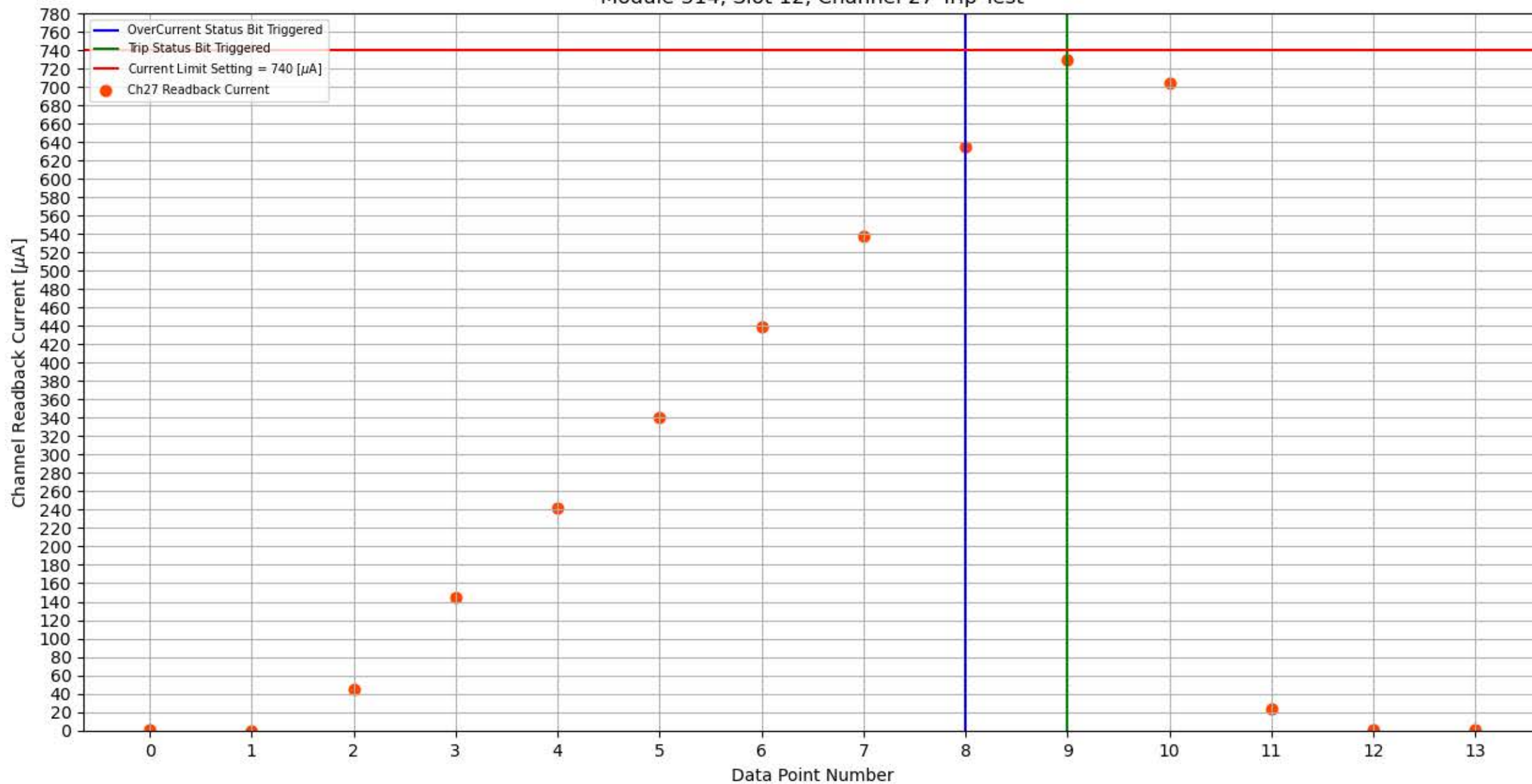
Module 314, Slot 12, Channel 27 Trip Test
