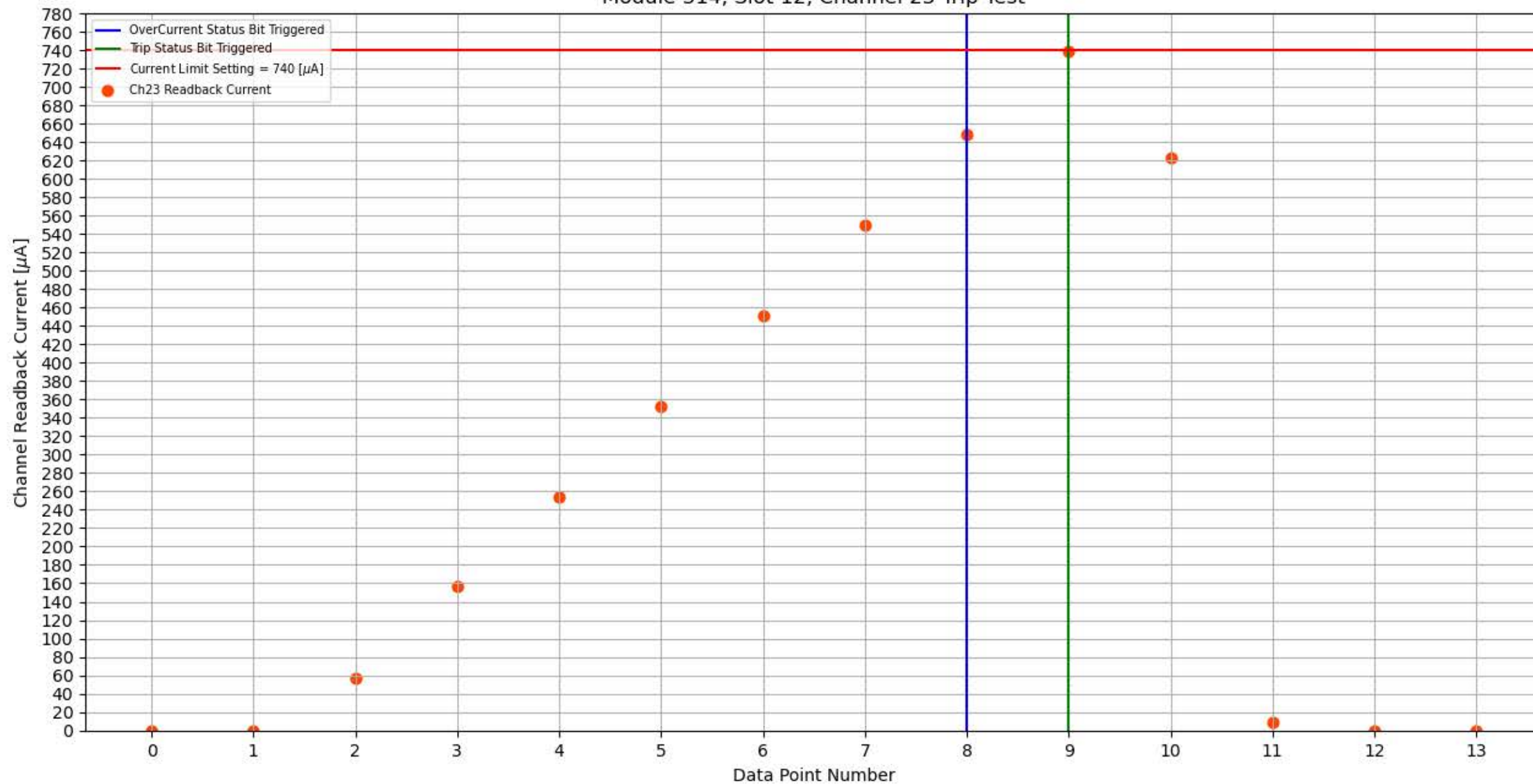
Module 314, Slot 12, Channel 23 Trip Test
