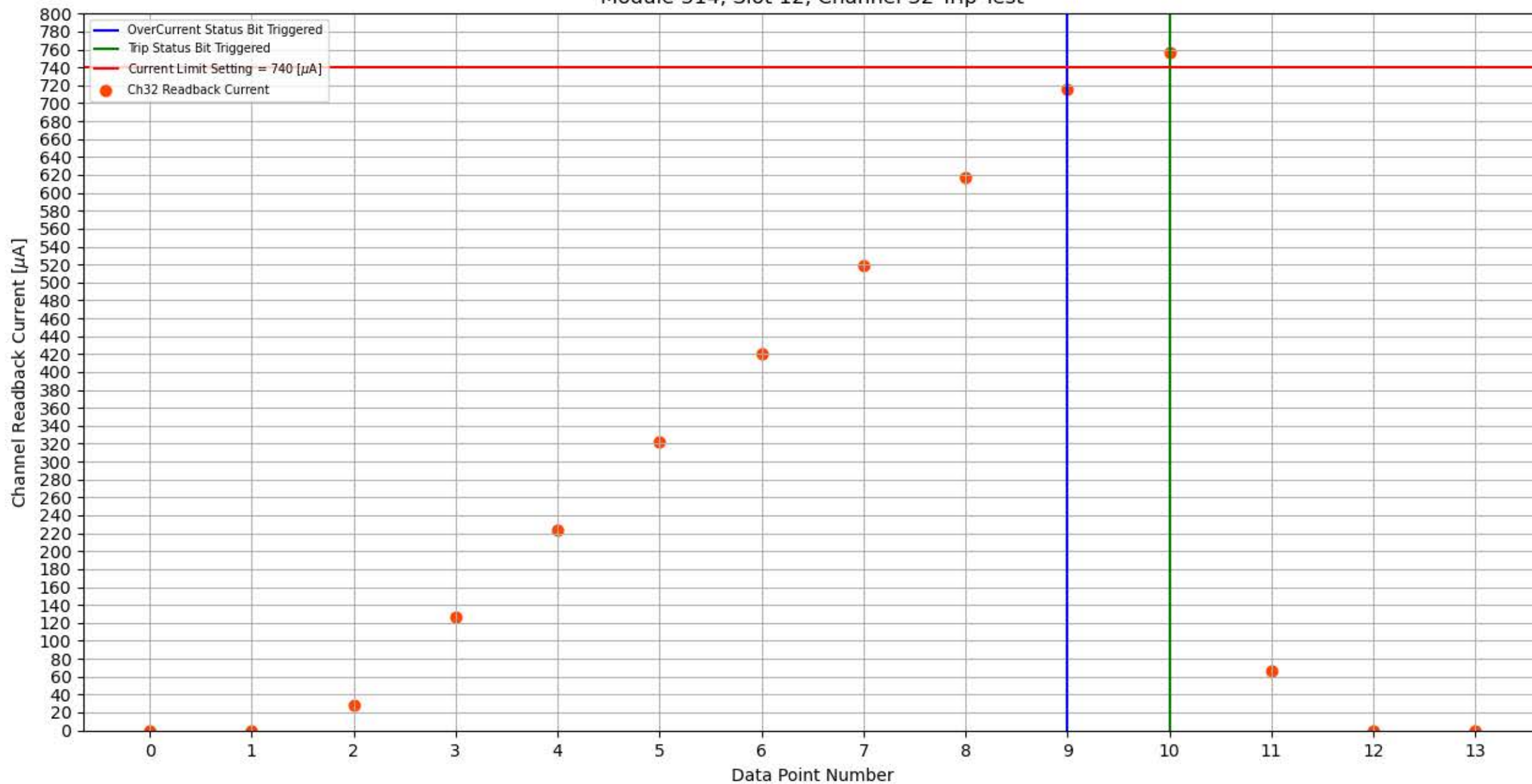
Module 314, Slot 12, Channel 32 Trip Test
