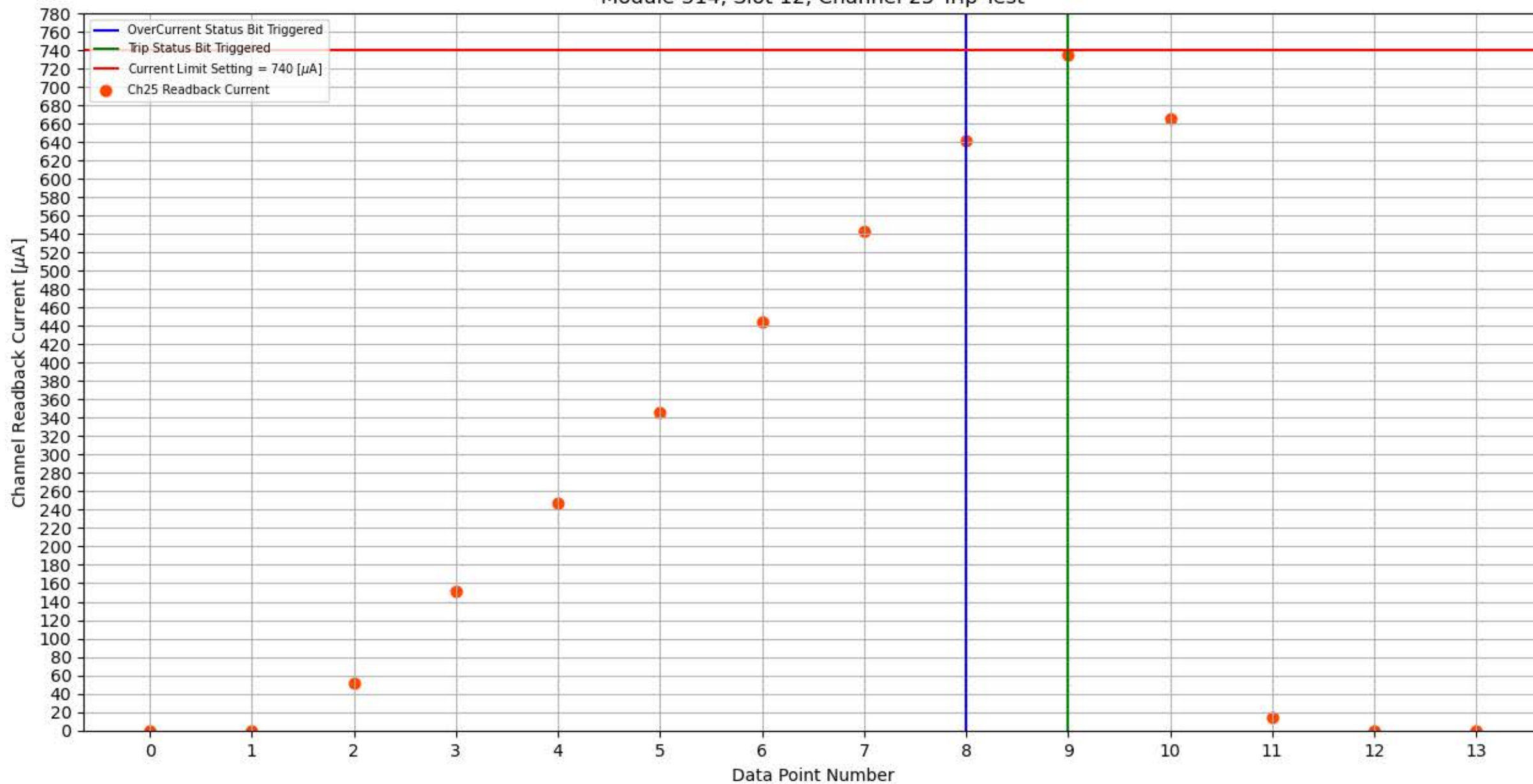
Module 314, Slot 12, Channel 25 Trip Test
