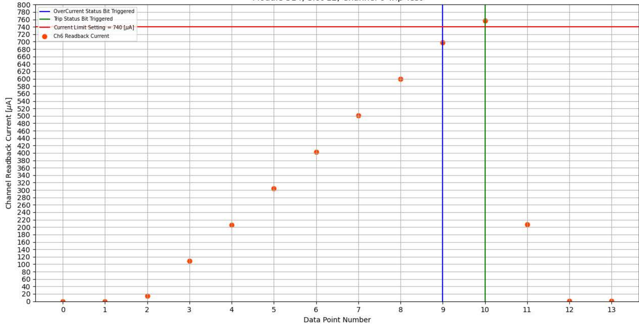
Module 314, Slot 12, Channel 6 Trip Test
