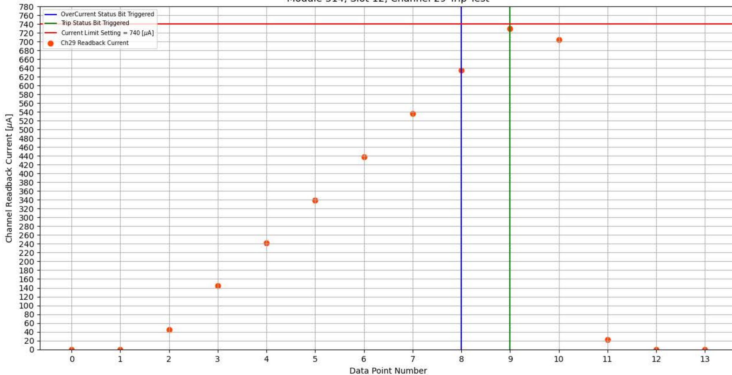
Module 314, Slot 12, Channel 29 Trip Test
