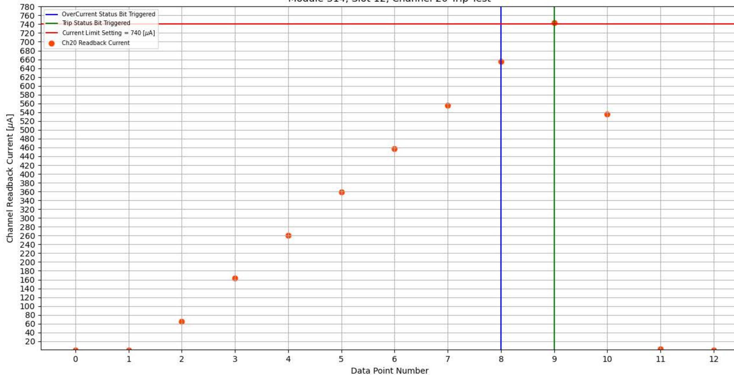
Module 314, Slot 12, Channel 20 Trip Test
