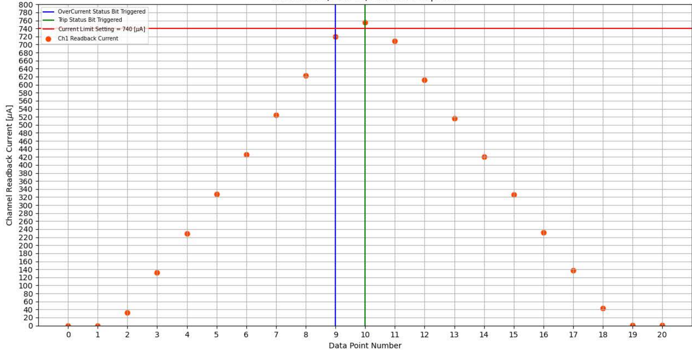
Module 314, Slot 12, Channel 1 Trip Test
