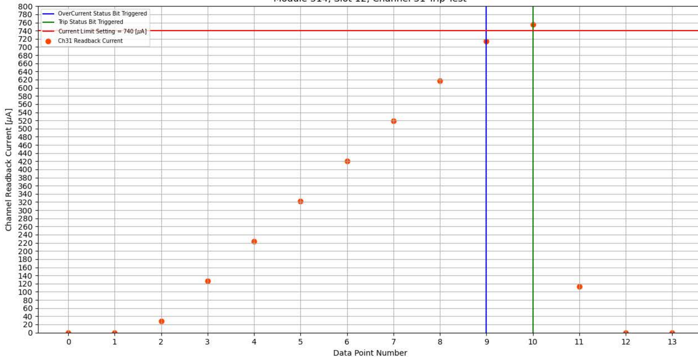
Module 314, Slot 12, Channel 31 Trip Test
