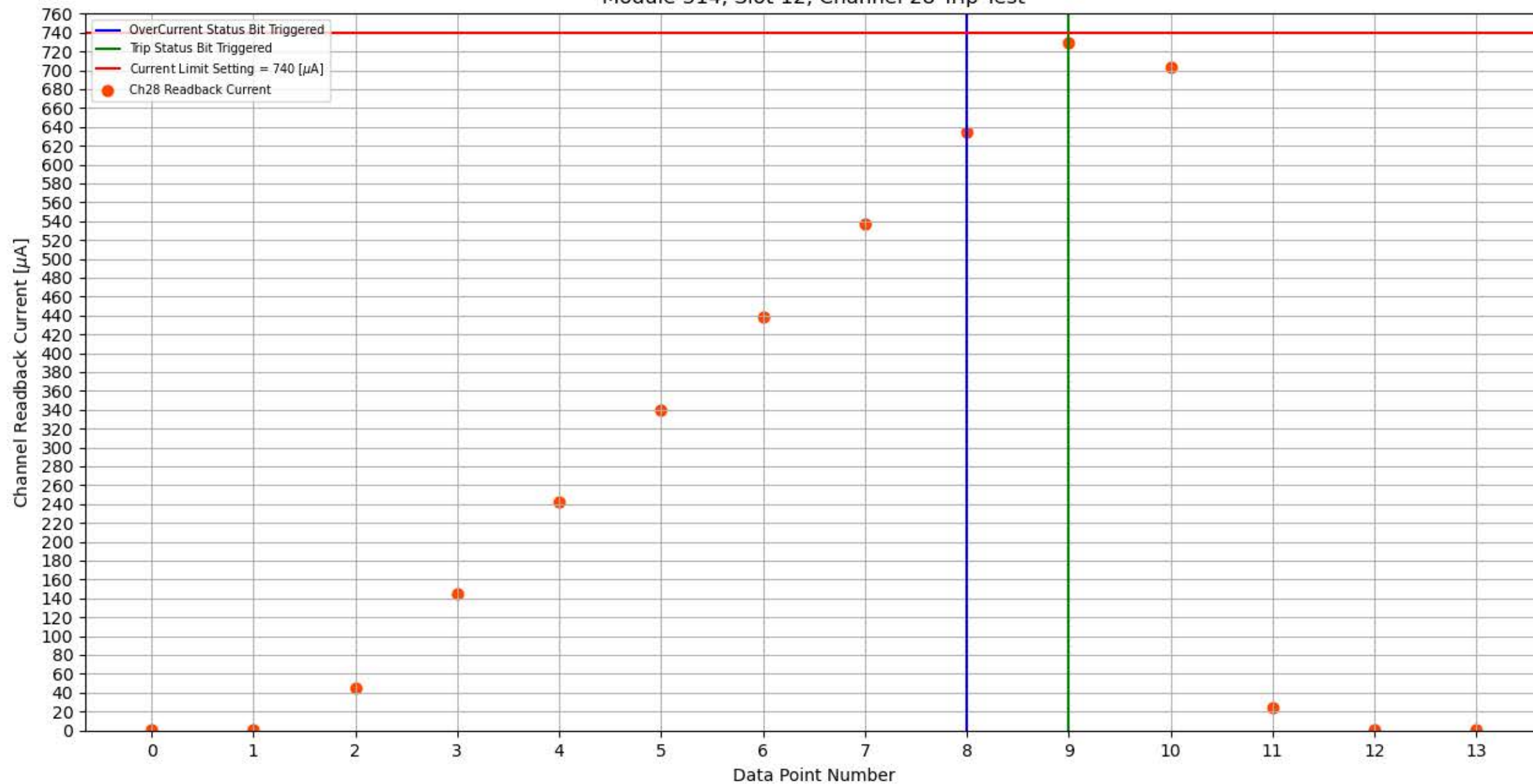
Module 314, Slot 12, Channel 28 Trip Test
